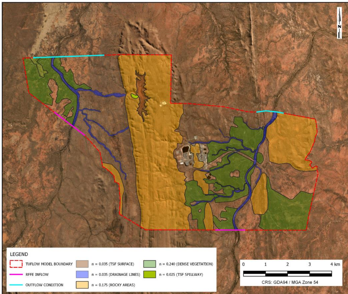
DIAGRAM 8: MANNINGS ROUGHNESS
