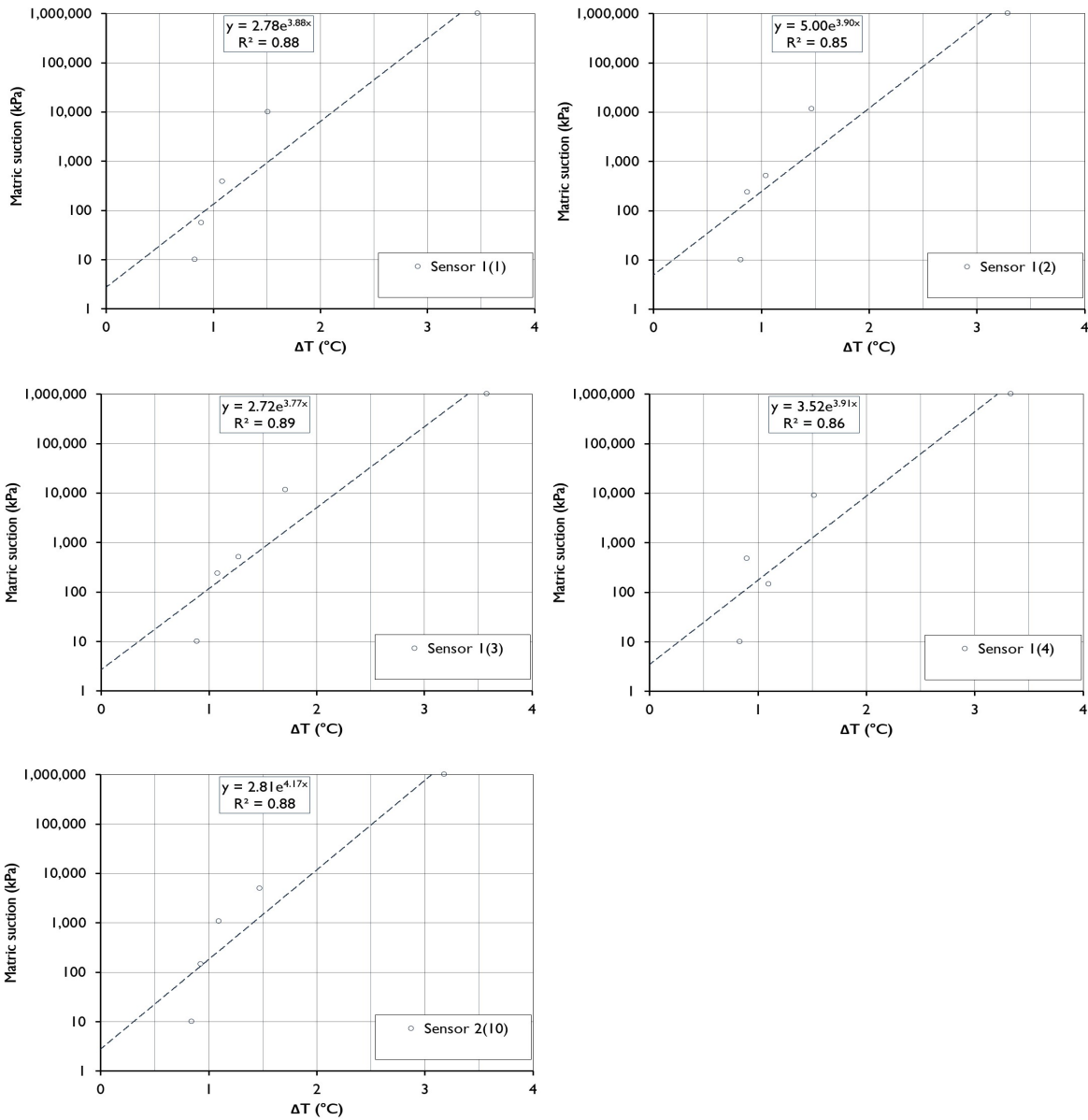
Figure 18 Cover option I matric suction sensor calibration curves
