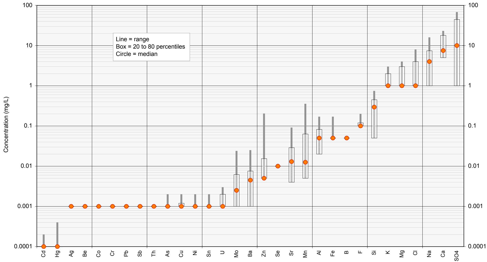
FIGURE 15: Statistical summary of AARC column leach assay data for samples comprising NAF Dugald River waste rock
