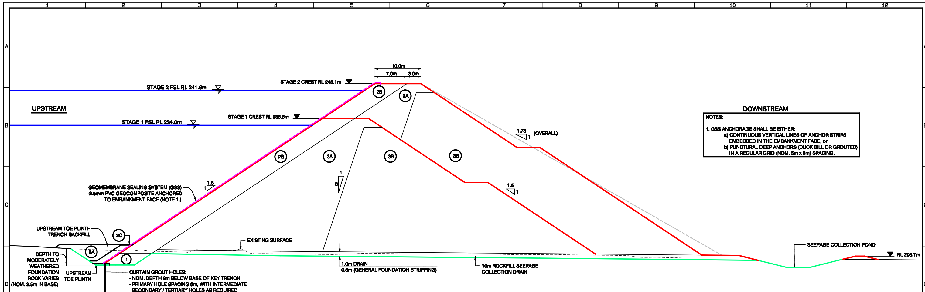
SECTION 1 MAIN EMBANKMENT (GSS OPTION) SCALE 1:500
